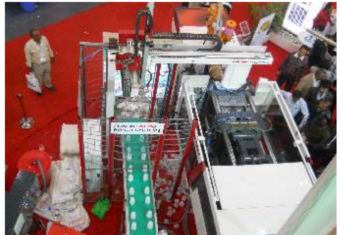
High Speed Servo Robot System on Injection Moulding Machine with Conveyor Belt and Safety Cage
